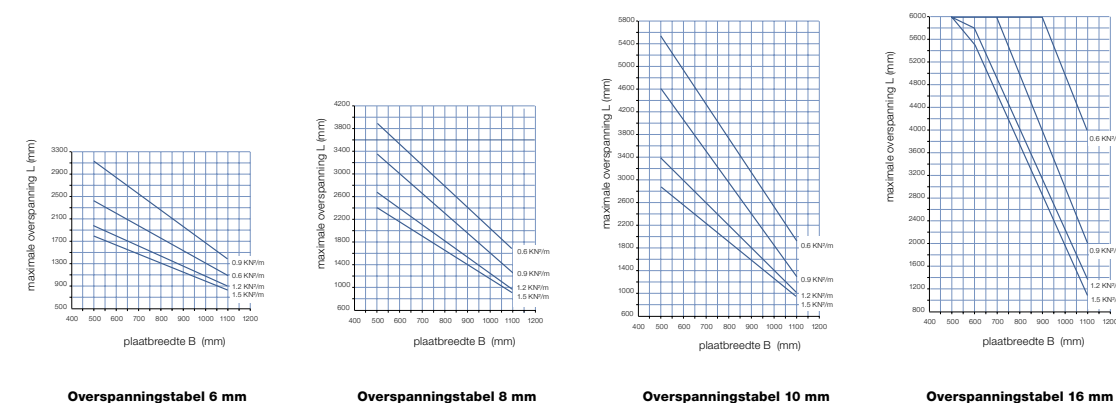
Overspanningstabel 6 mm Overspanningstabel 8 mm Overspanningstabel 10 mm Overspanningstabel 16 mm
